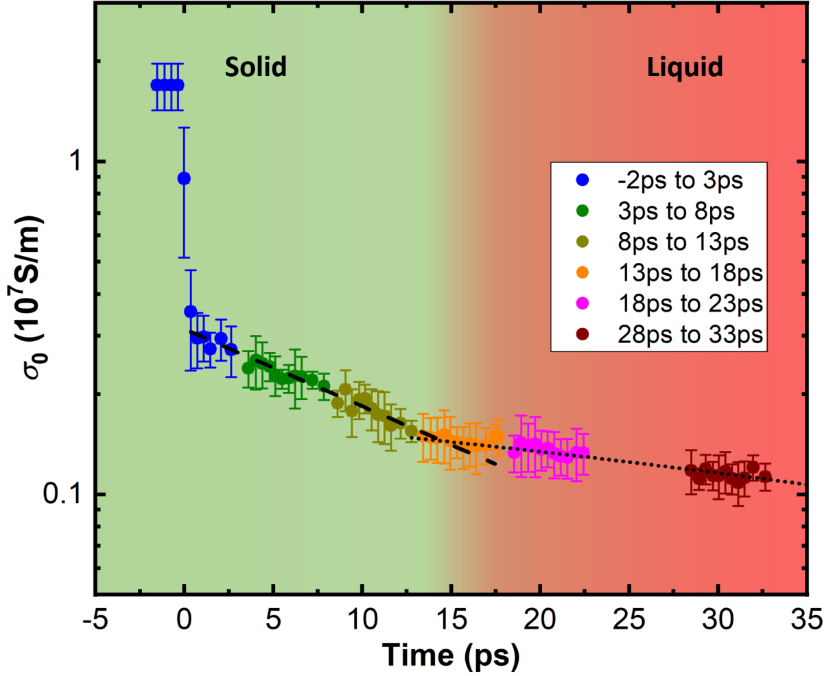
Figure 4: Time-resolved electrical conductivity \sigma_0 of gold (logarithmic vertical axis) at mean excitation energy density of 0.89 \pm 0.18 MJ/kg measured by multi-cycle THz-FEL at various time delays. Each section covers a time interval of 5 ps and the data present an averaged over 4-6 shots. The error-bars include the standard deviation and the systematic error of the measurements. The data after 0 ps are fit by a two-segment exponential decay function represented by the dashed and the dotted lines. The intersection of these two curves at t = 14.5 ps coincides with the melting phase transition of gold.
